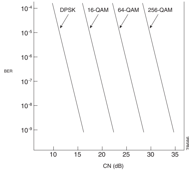
Figure 20-1 Error Rates for PSK and QAM Systems
