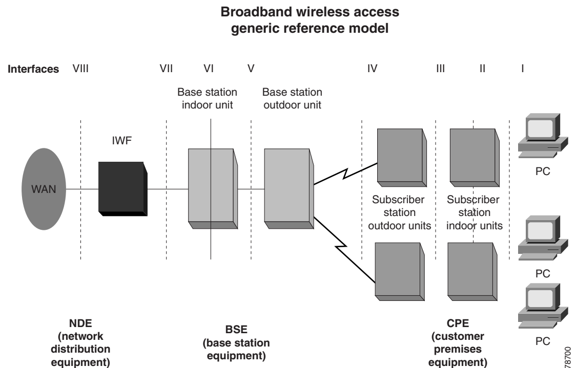
Figure 20-15 Generic Reference Model for Broadband Wireless Access
