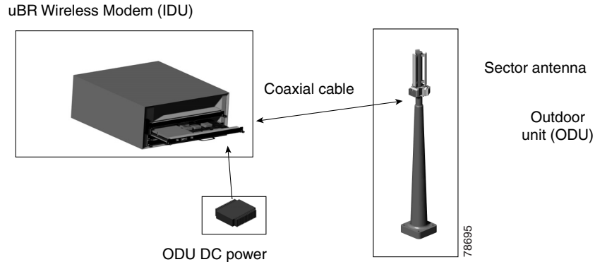
Figure 20-10 The Cisco MMDS Broadband Wireless Access System
