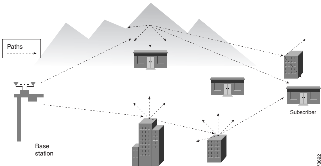
Figure 20-7 Typical Multipath Example
