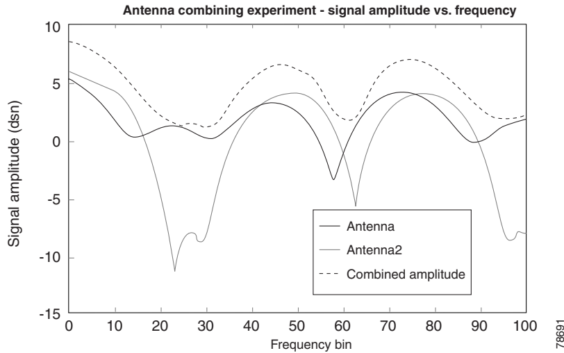
Figure 20-6 Multipath Reception
