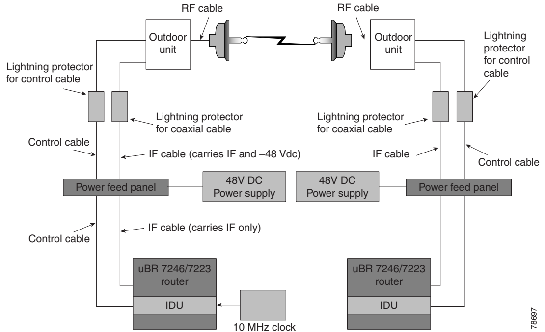
Figure 20-13 Open Standard Wireless Architecture
