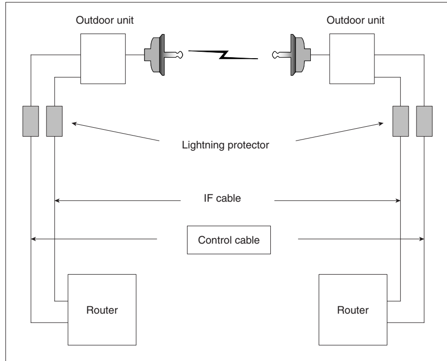
Figure 20-5 Spectrum Technology
